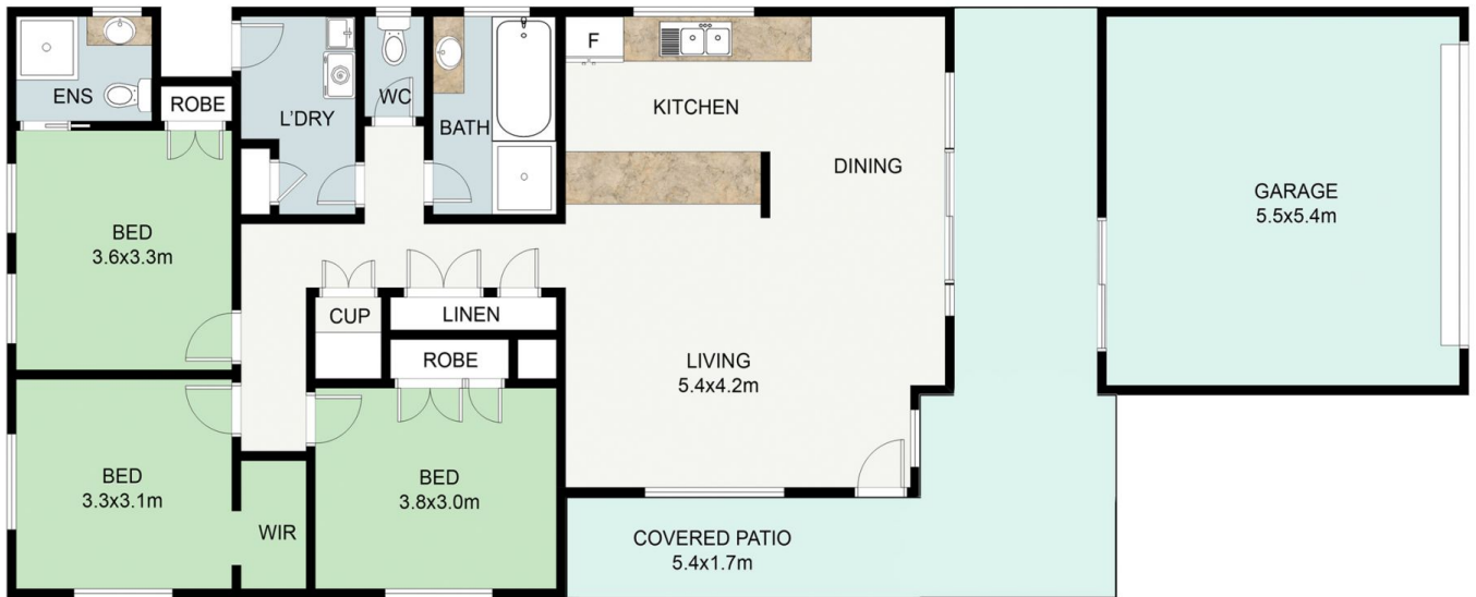
FLOOR PLAN
