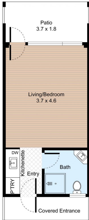
FLOOR PLAN
